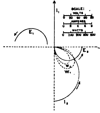
FIG. 6.—Constant Current, Step Down, Arm at 70^\circ
